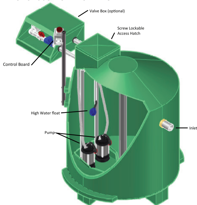
SPS4000 PUMP STATION
