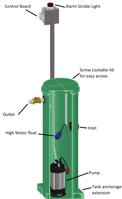
SPS300 PUMP STATION
